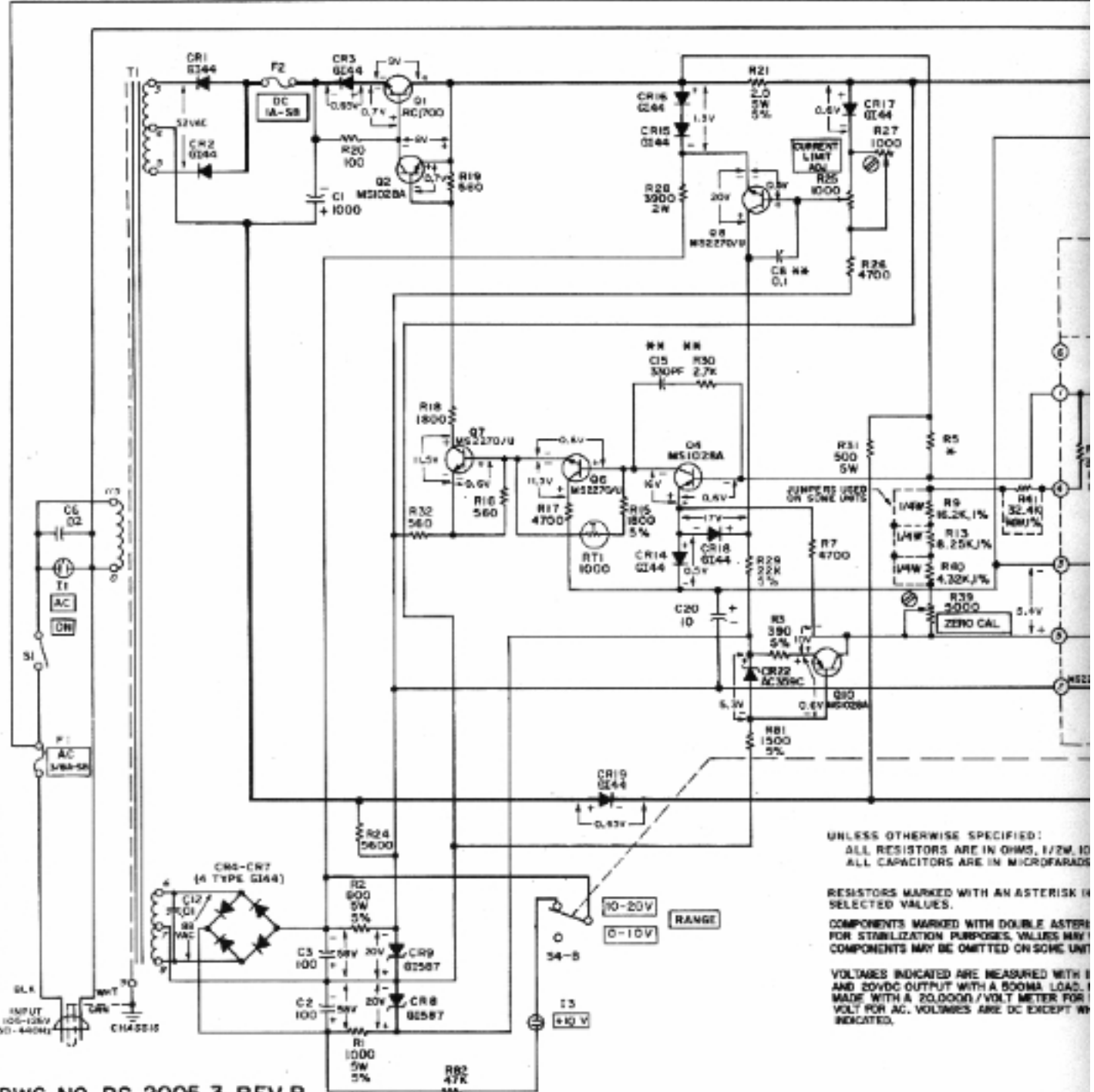
DWG. NO. PS-2005-3 REV. R MODEL 2005 TRANSISTORIZED POWER SUPPLY
