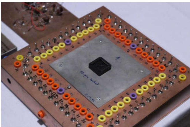
Prototypes from Bob Pease's home, given away by TI.
