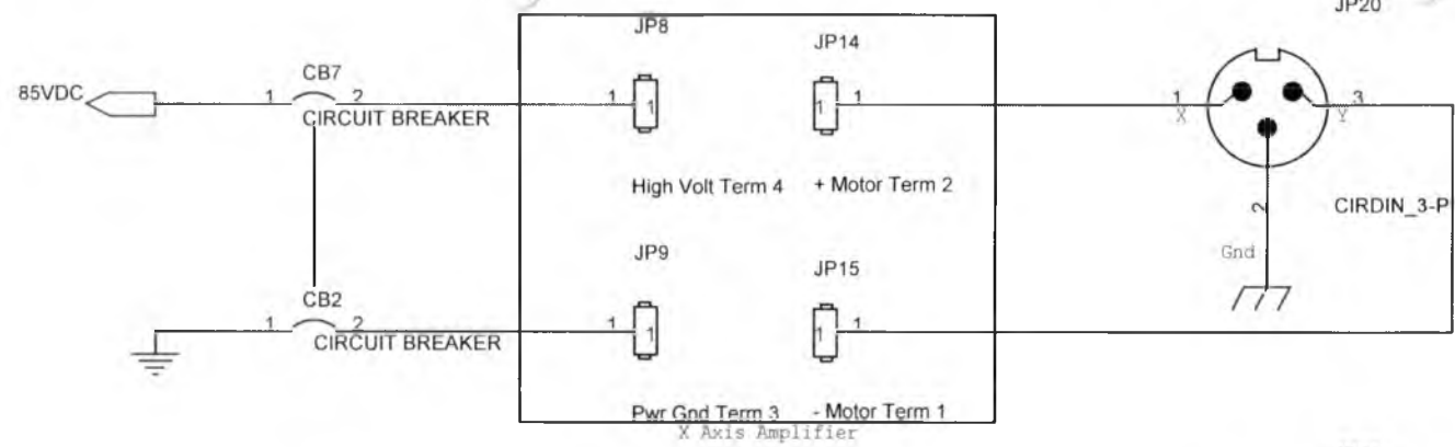
X Axis Amplifier
