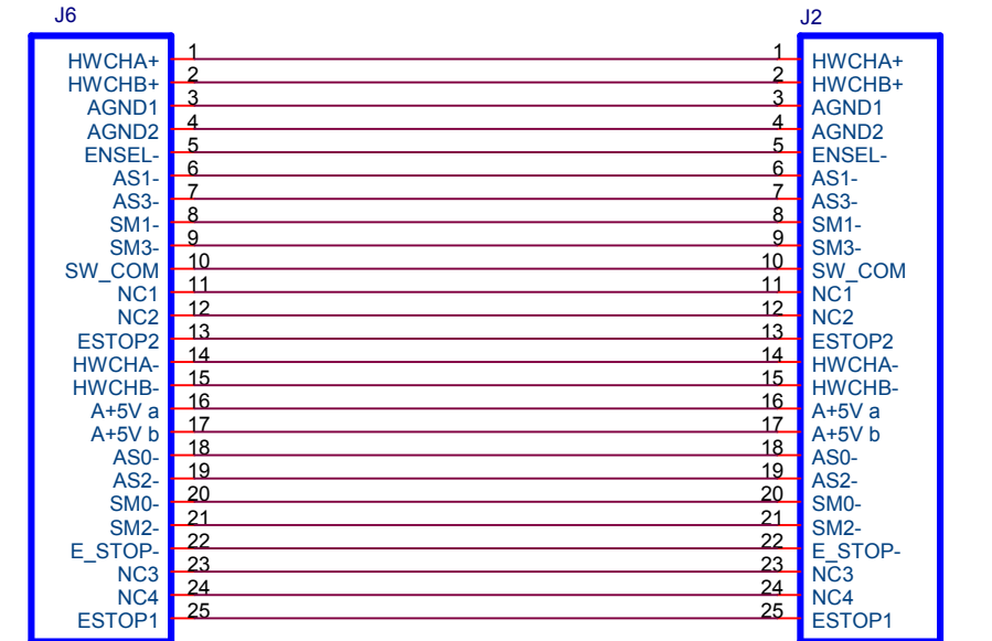
J6 Remote Handwheel
